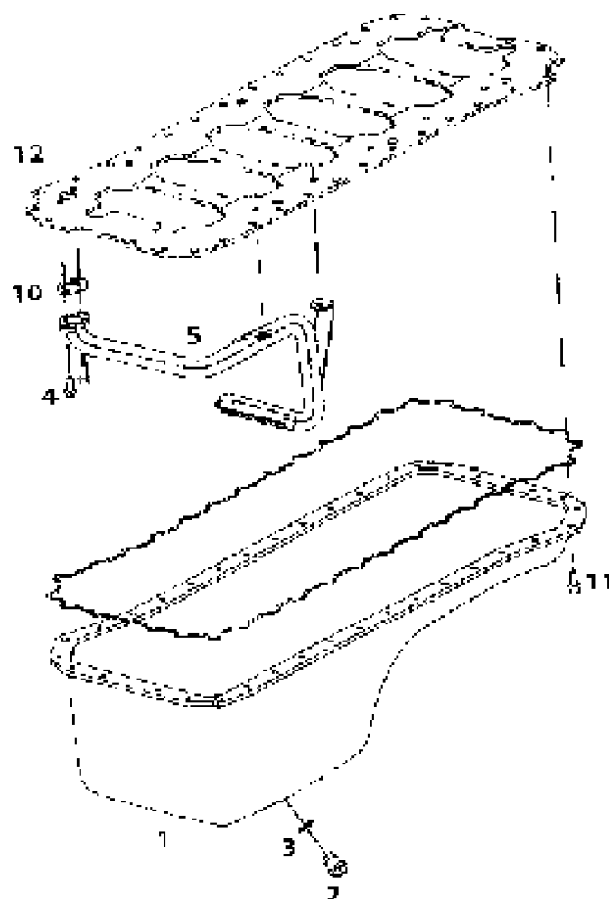
OIL PAN
