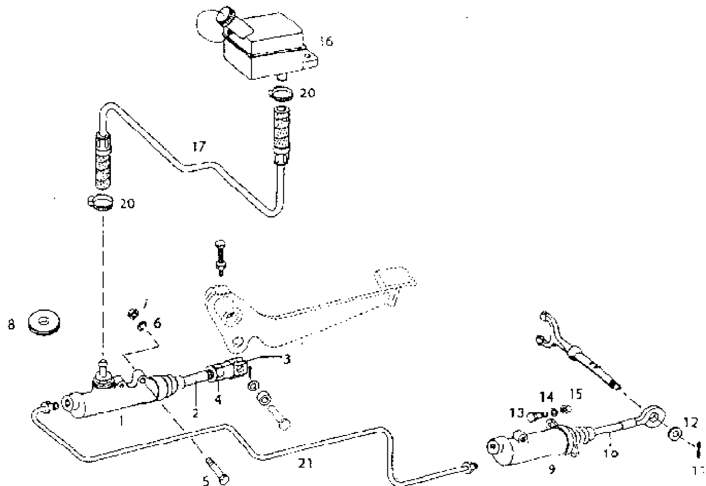
HYDRAULIC CLUTCH CONTROL
