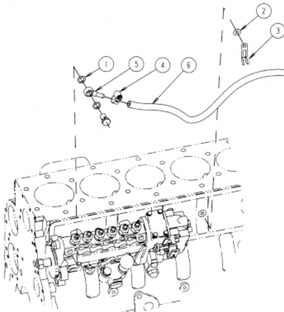
LOCATION FUEL DRAIN
