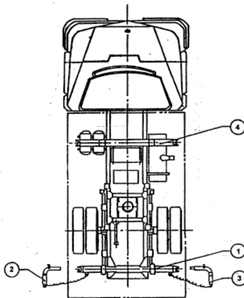
STABILITY SHAFT
