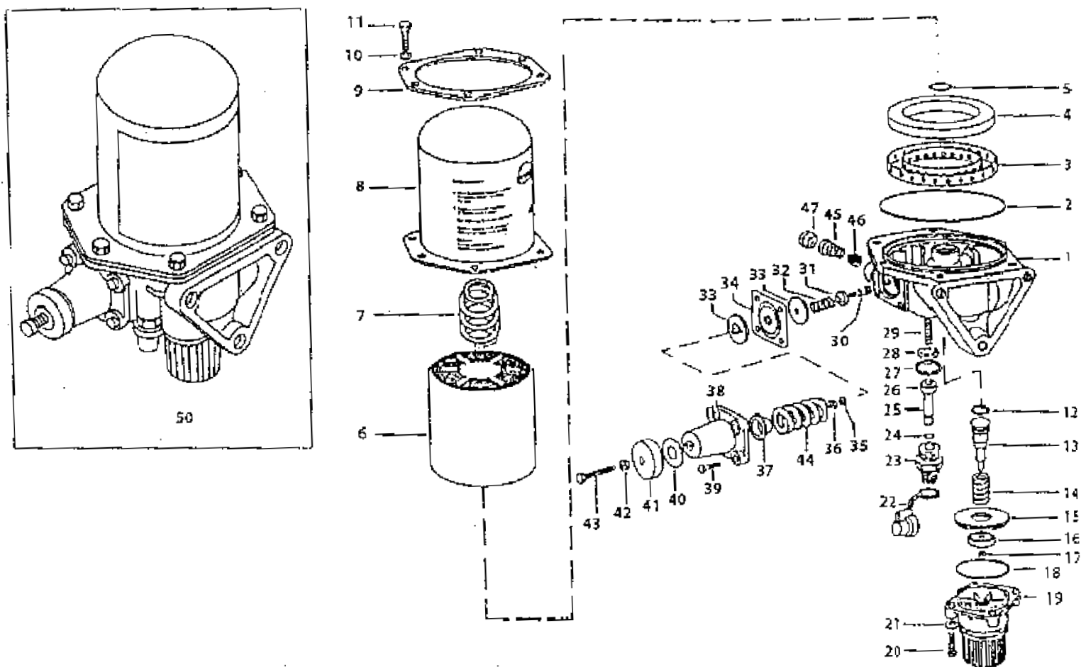
AIR DRYER
