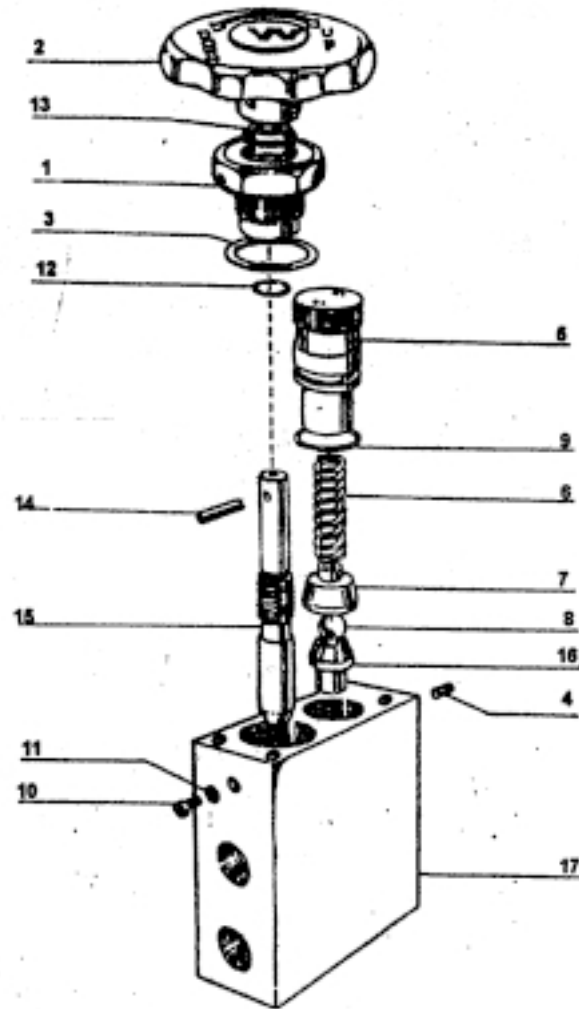
MANUAL VALVE ROTARY
