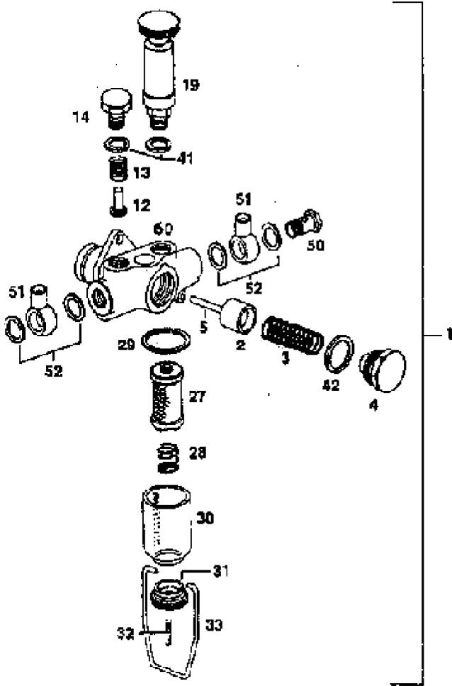
FUEL FEED PUMP
