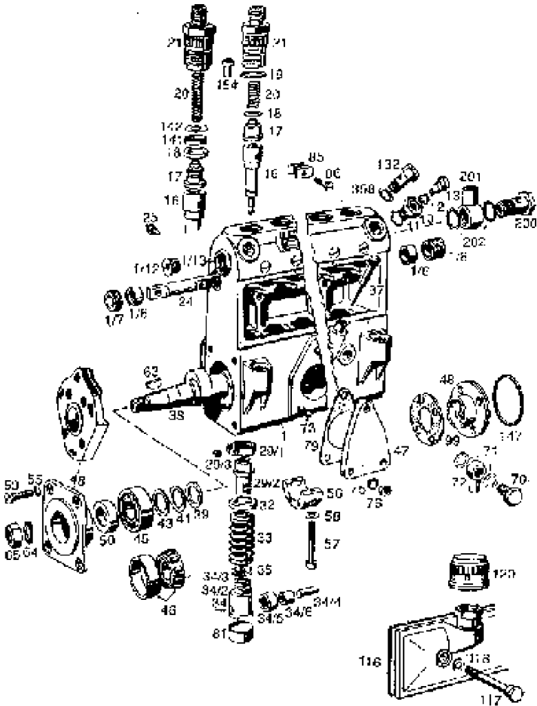
FUEL INJECTION PUMP
