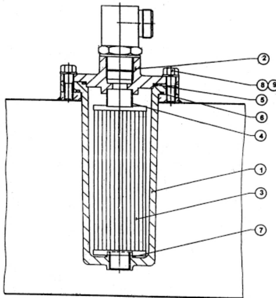
RETURN LINE FILTER
