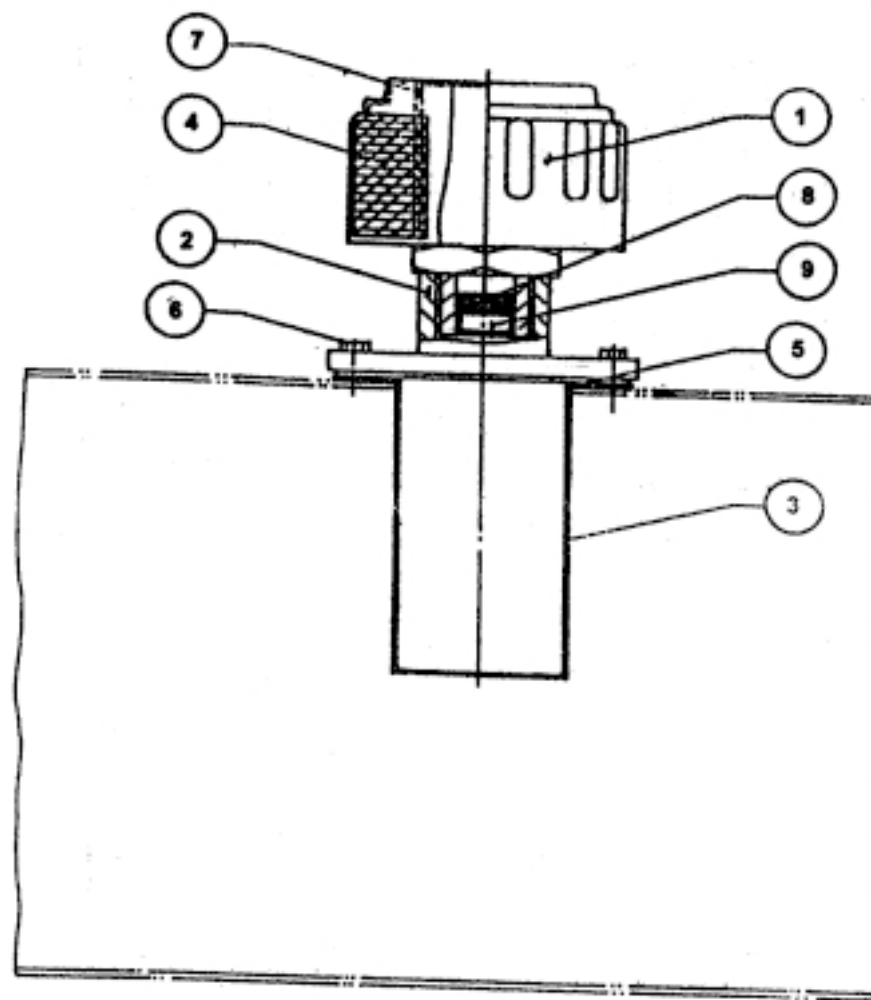
FILTER BREATHER
