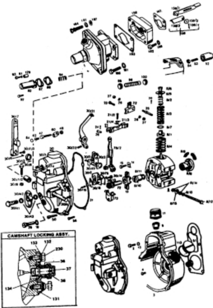
RQV GOVERNOR
