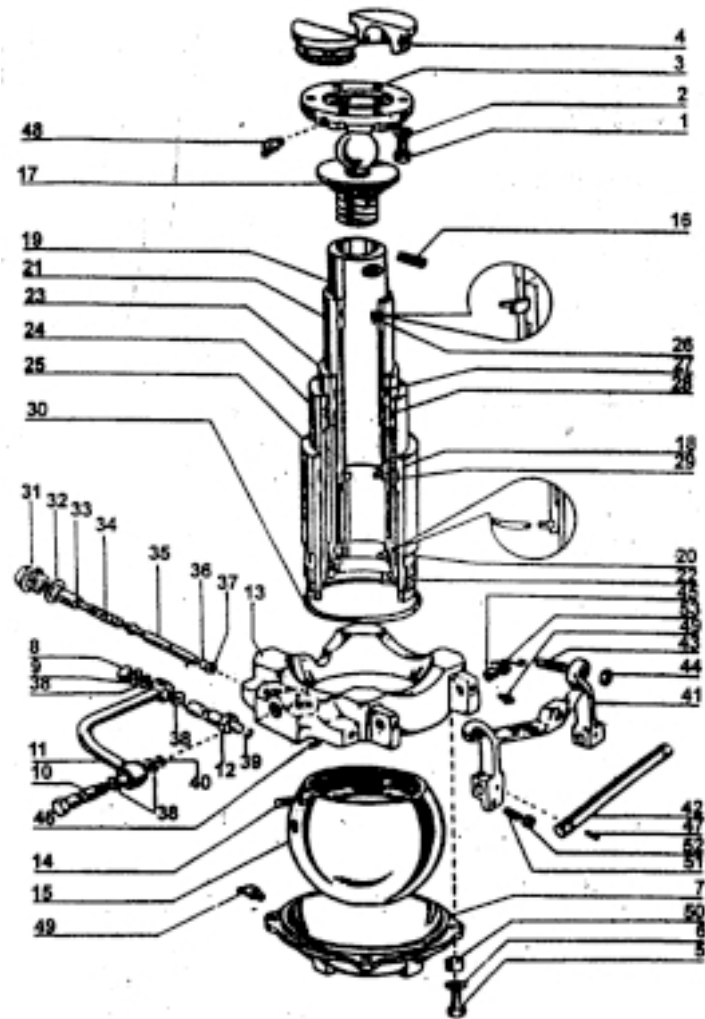
TELESCOPIC CYLINDER (4 STAGE)
