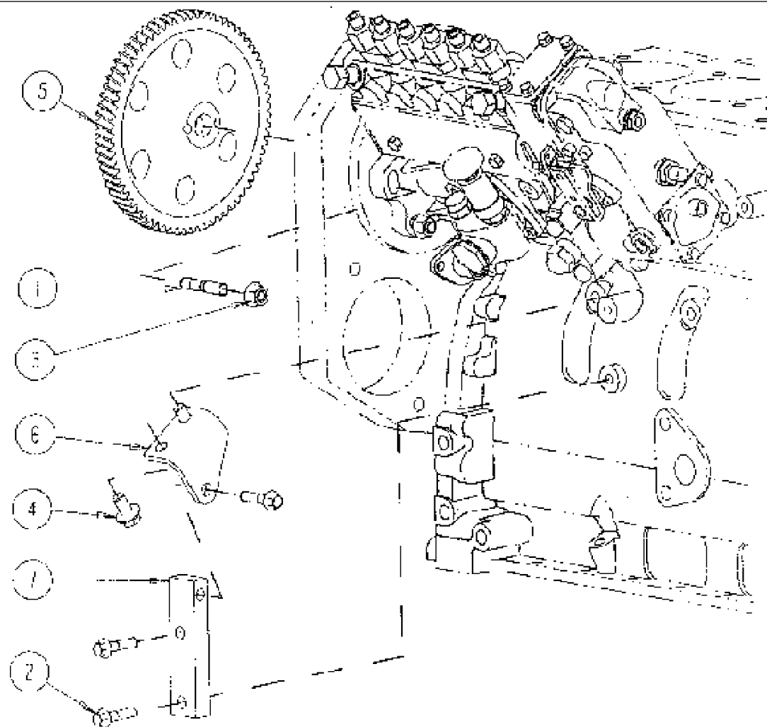
FUEL PUMP COUPLING
