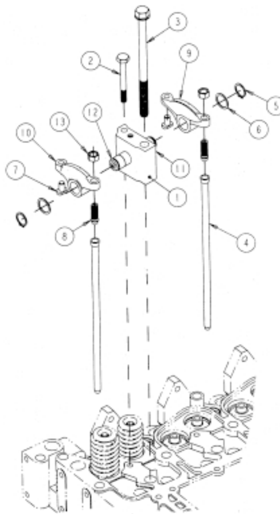
ROCKET LEVER
