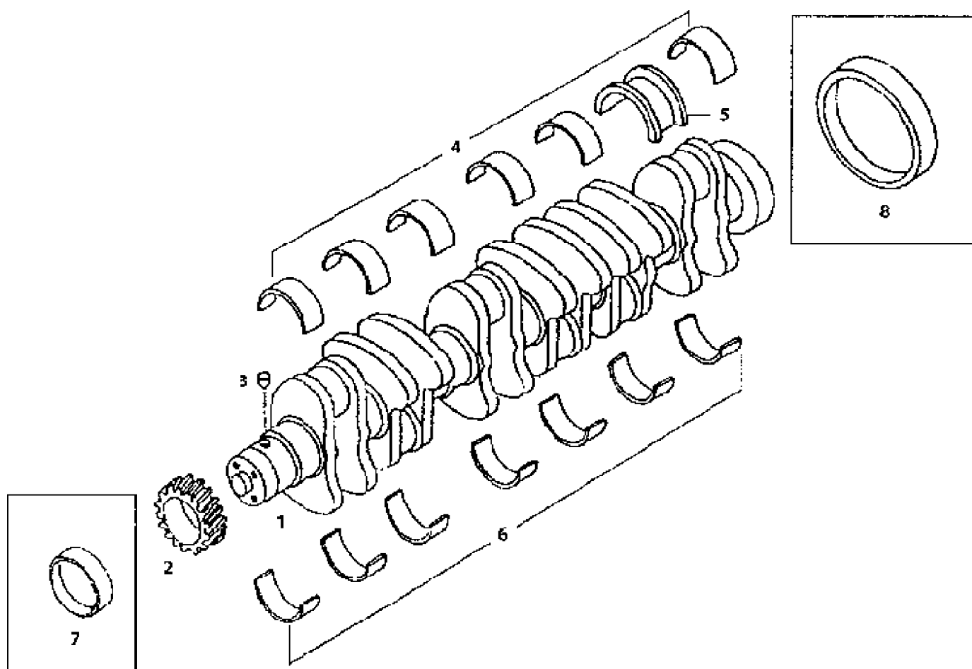
CRANKSHAFT AND MAIN BEARING
