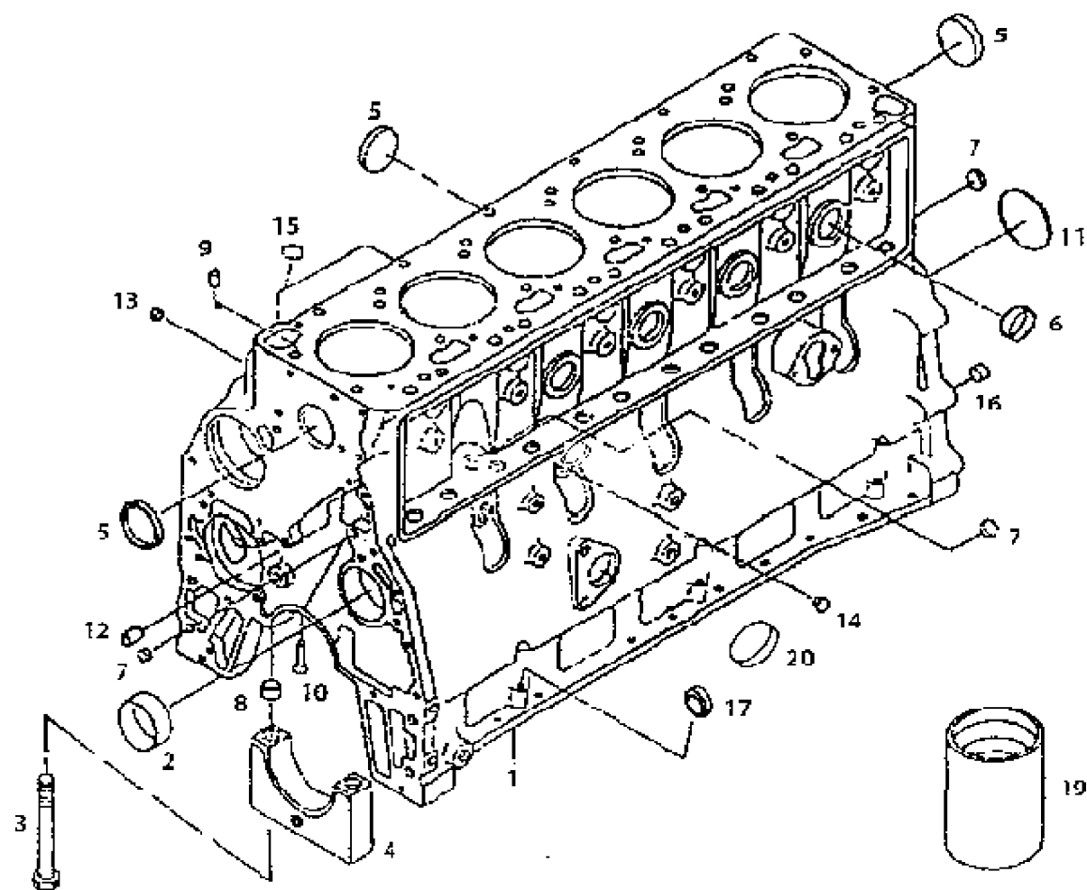
CYLINDER BLOCK
