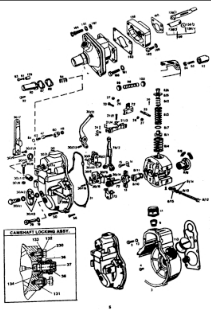
RQV GOVERNOR
