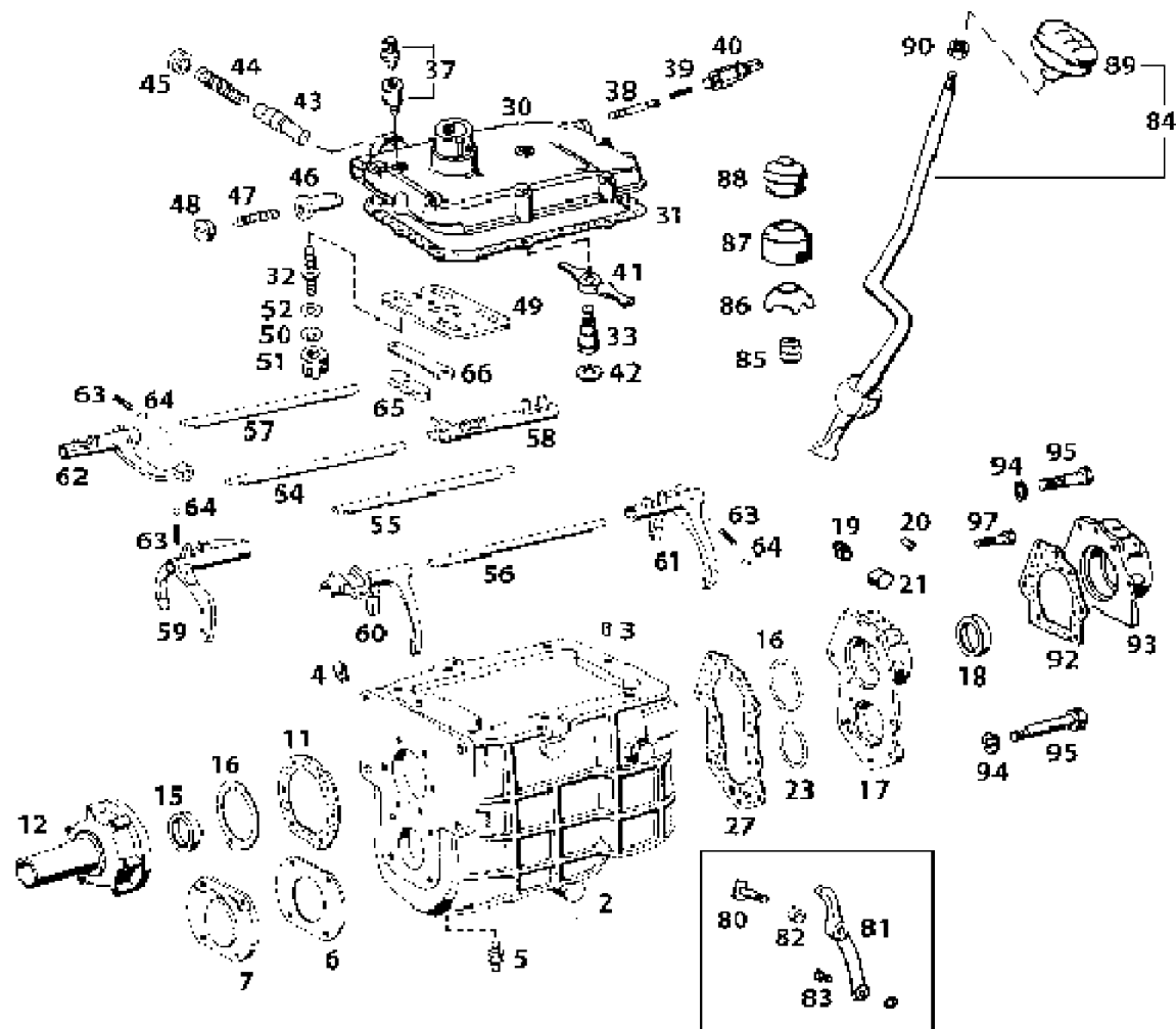
GBS 40 SYNCHROMESH TRANSMISSION
