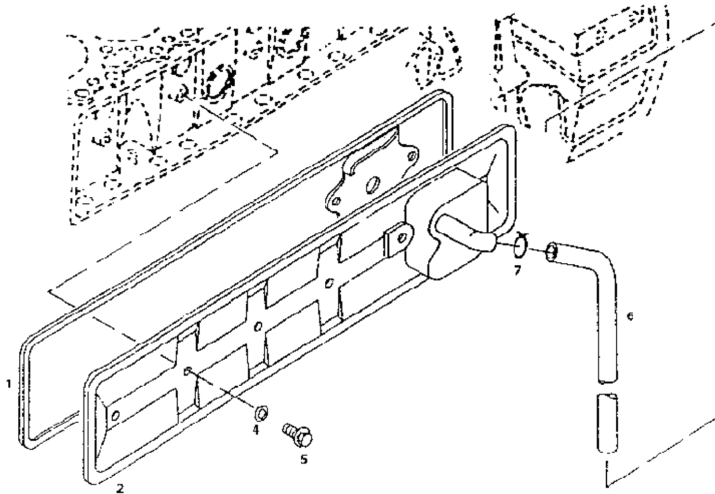
CAM FOLLOWER COVER
