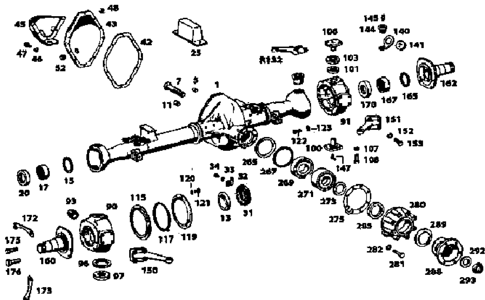
FRONT AXLE
