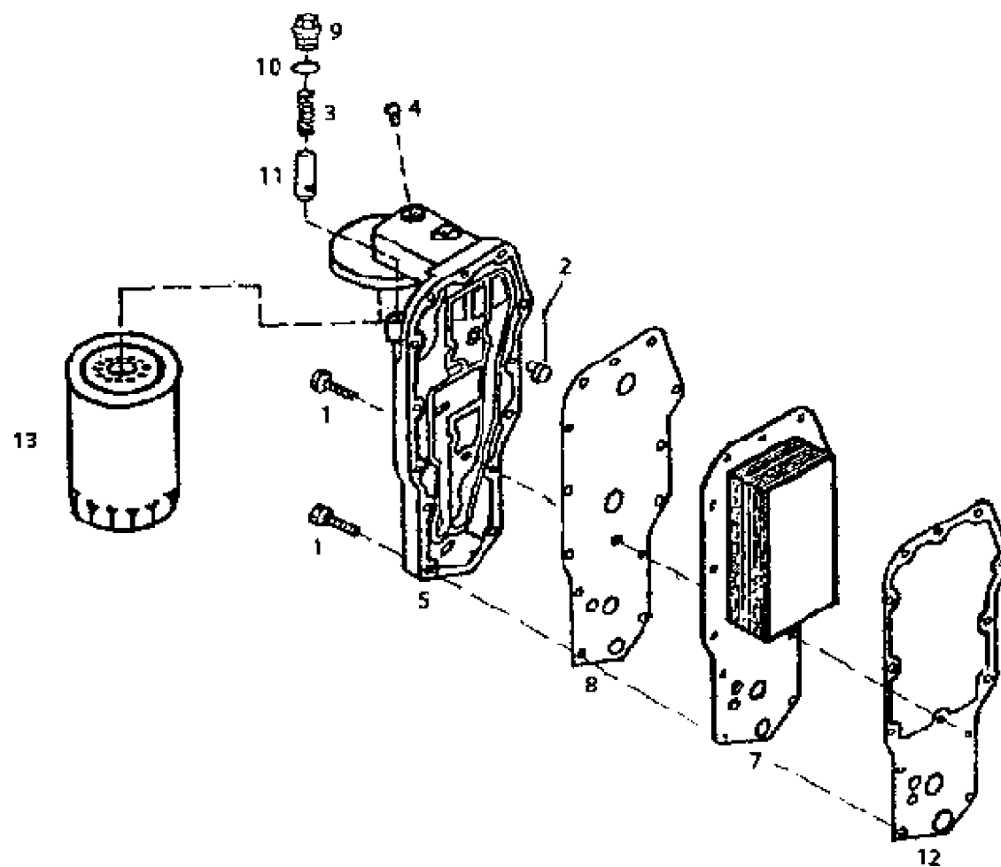
LUBRICATING OIL COOLER / OIL FILTER
