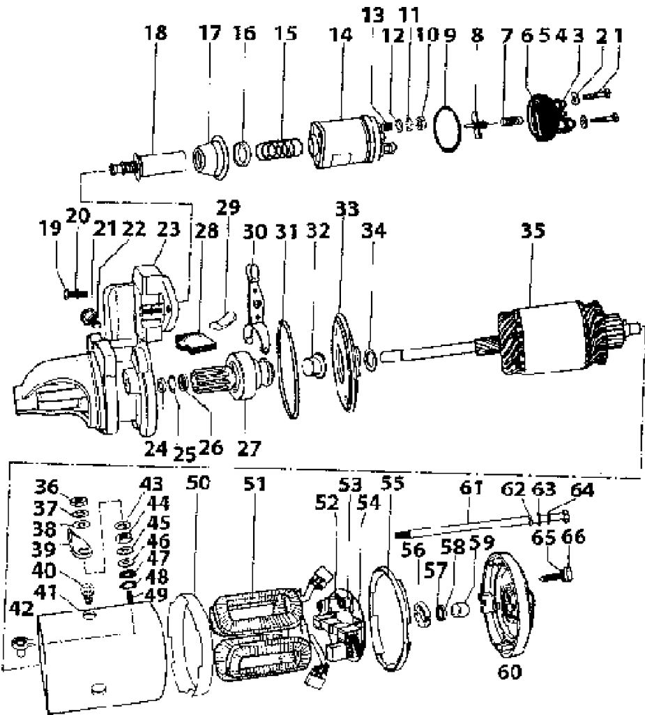
COMPONENT DETAILS OF STARTER MOTOR
