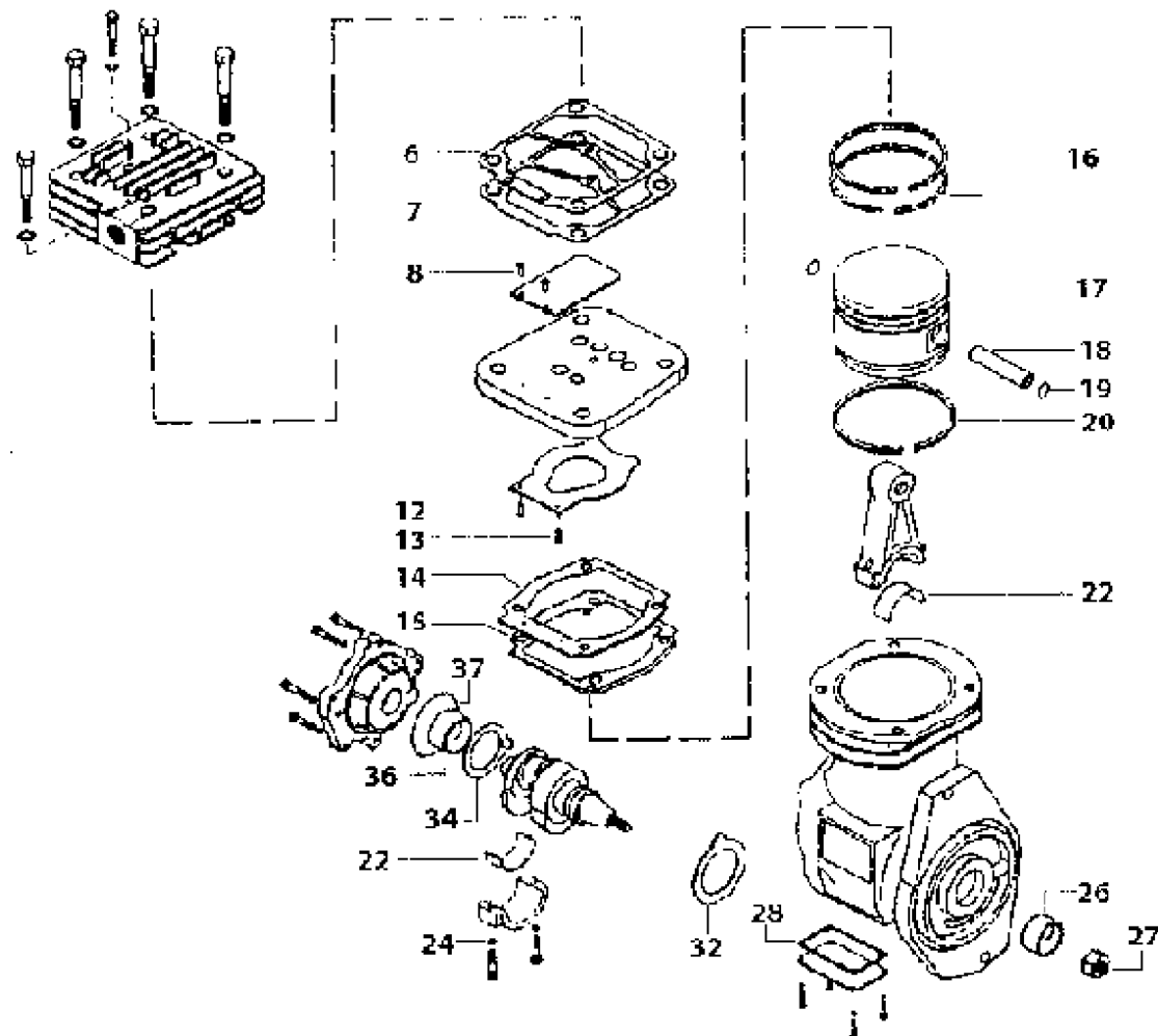
KIT FOR AIR COMPRESSOR
