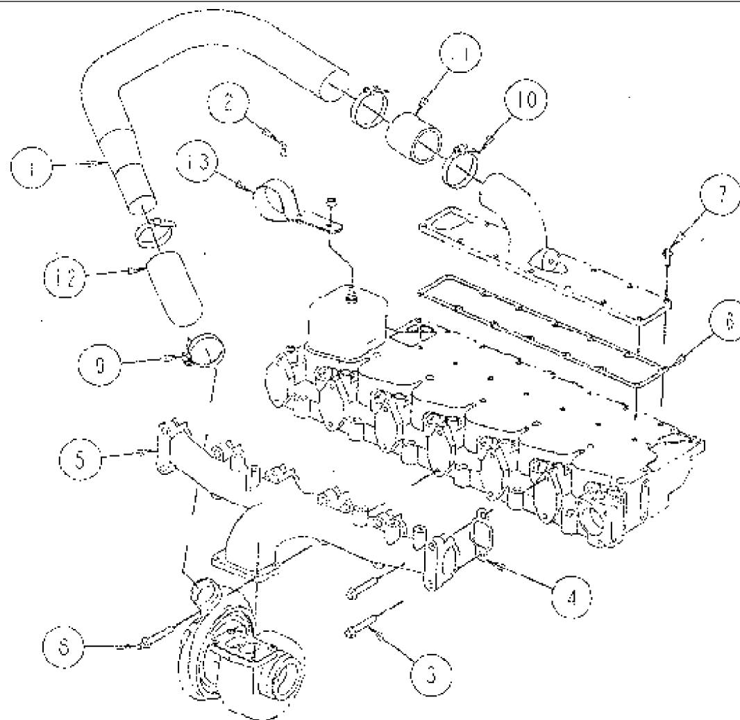
LOCATION TURBOCHARGER AND MANIFOLD
