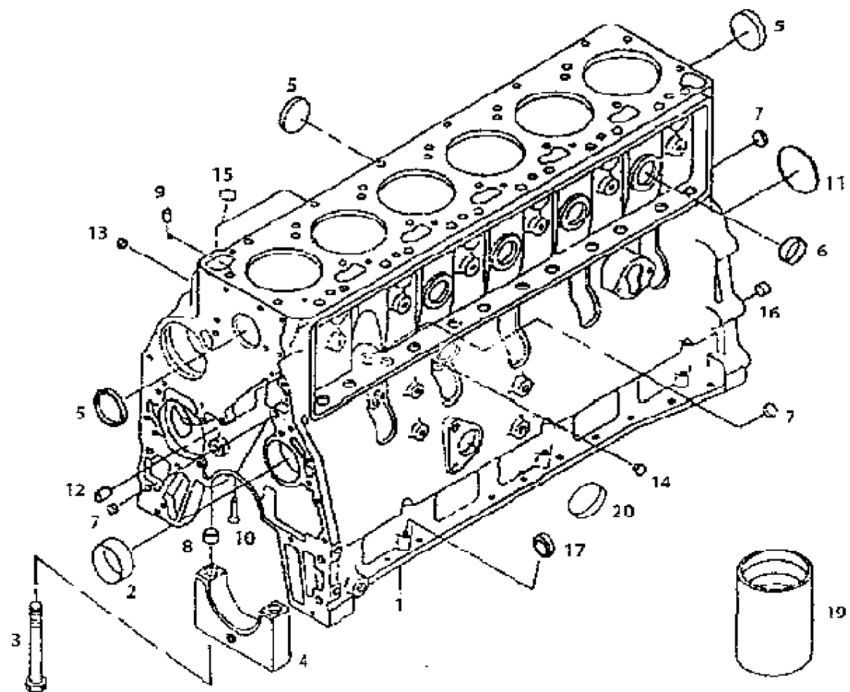
CYLINDER BLOCK
