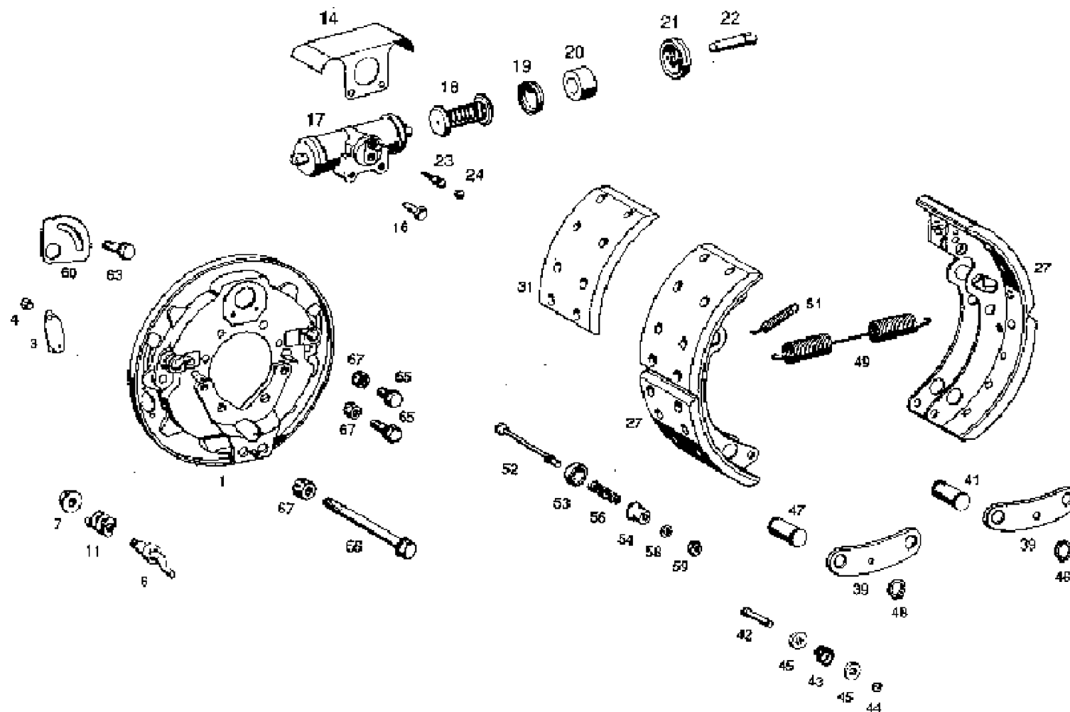
FRONT WHEEL BRAKE
