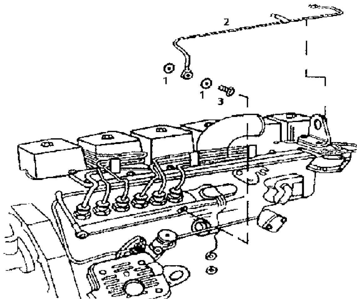
FUEL FILTER PLUMBING
