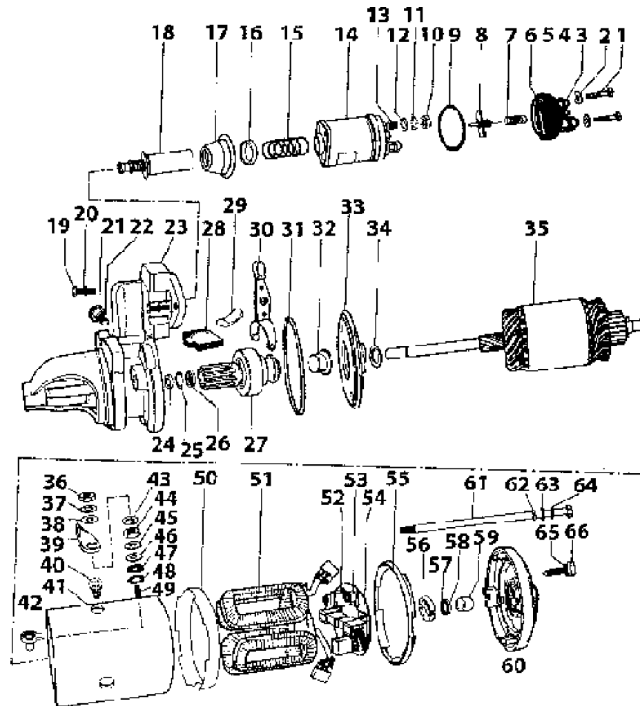
COMPONENT DETAILS OF STARTER MOTOR
