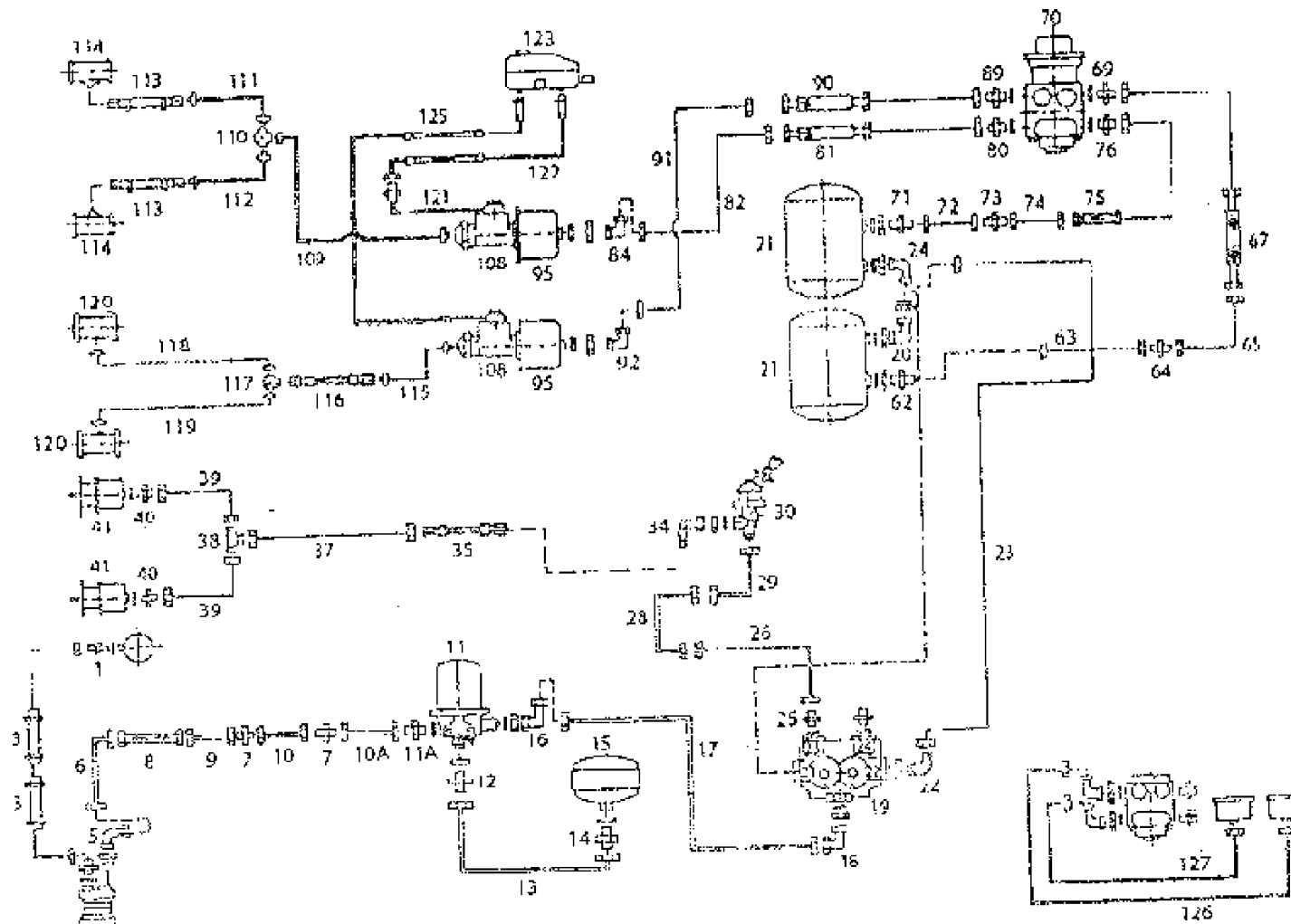
BRAKE LINES
