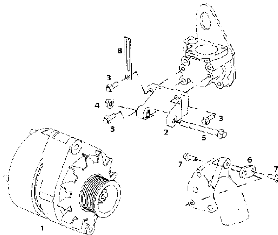
ALTERNATOR & ALTERNATOR LOCATION
