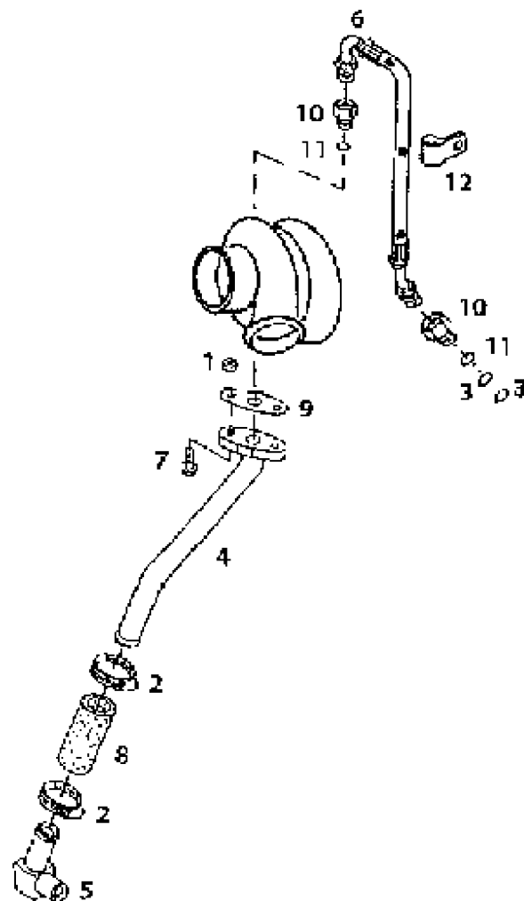
PLUMBING TURBOCHARGER
